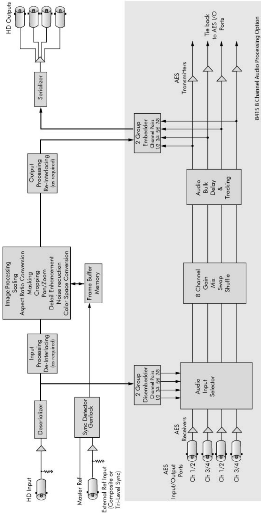
7930 HD Cross Converter Functional Block Diagram, Landscape View
