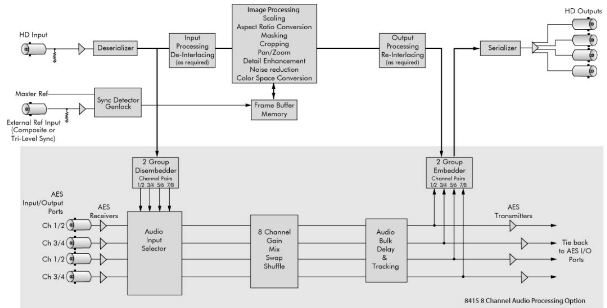
7930 HD Cross Converter Functional Block Diagram, Portait View
