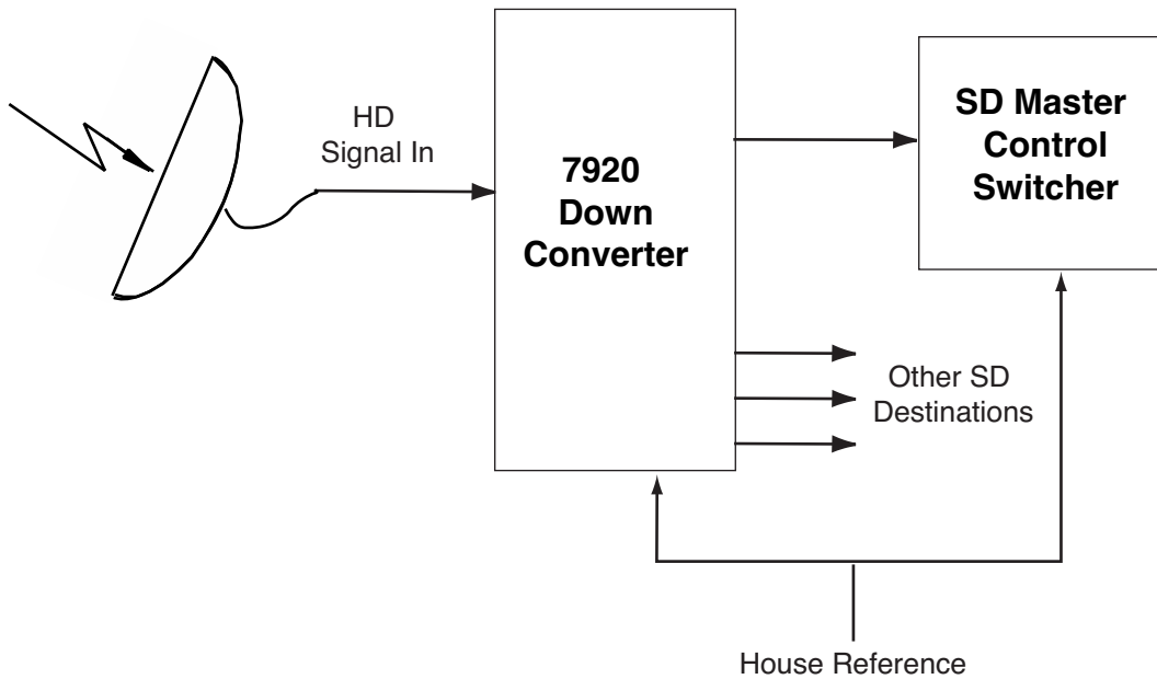
7920 HD Downconverter Application
