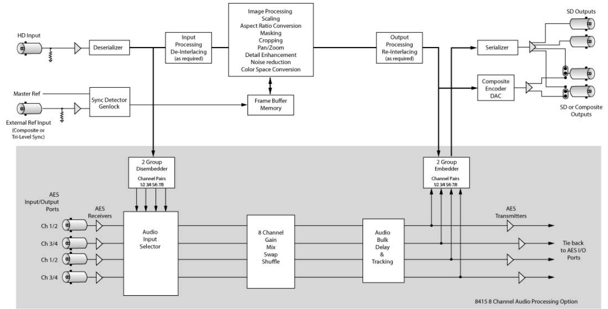
7920 HD Downconverter Functional Block Diagram, Portrait View
